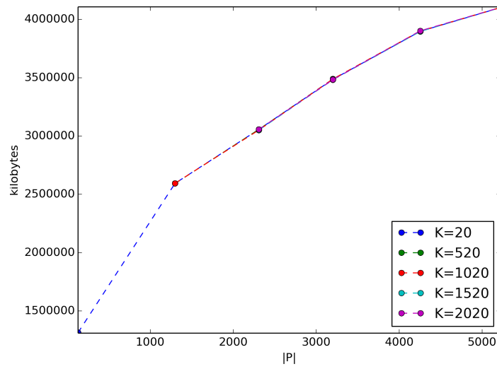
Fig. 14: Maximum memory used vs. |P| . Greenland dataset
