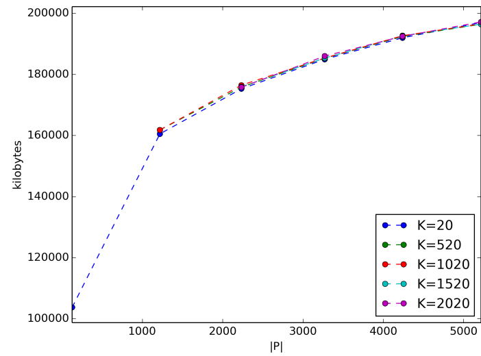
Fig. 10: Maximum memory used vs. |P| for C10D50K-A2B2-N3
