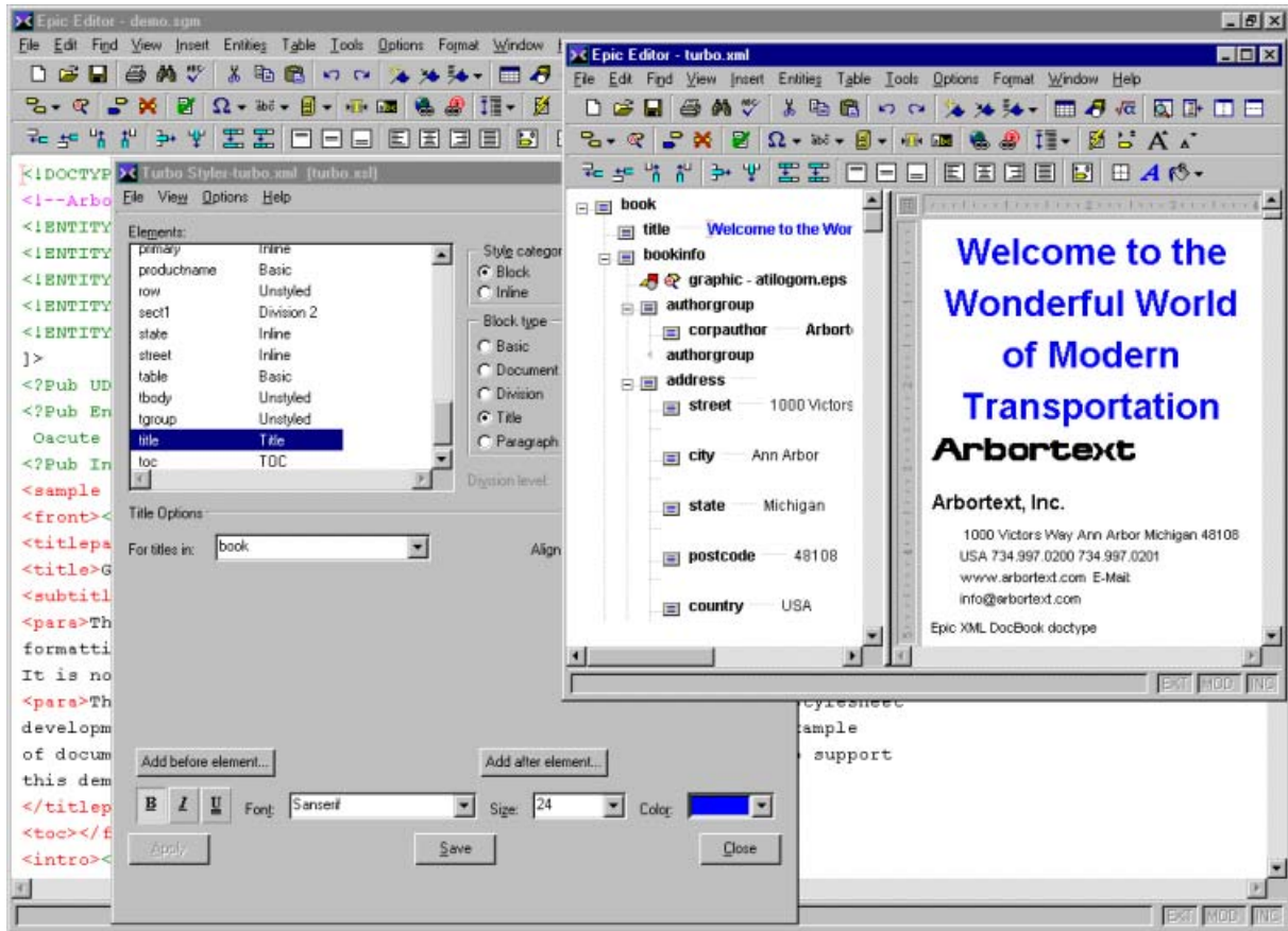
Figure 31 : Epic Editor
