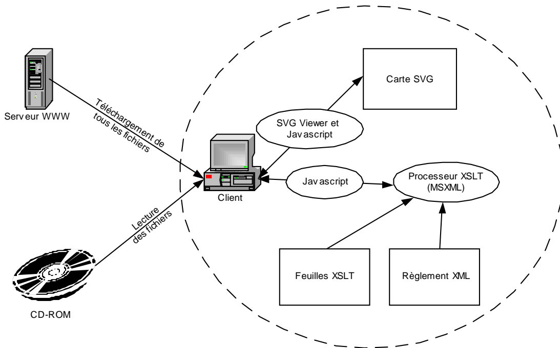
Figure 20 : Architecture "application locale"
