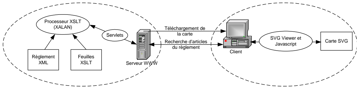
Figure 21 : Architecture "client léger "
