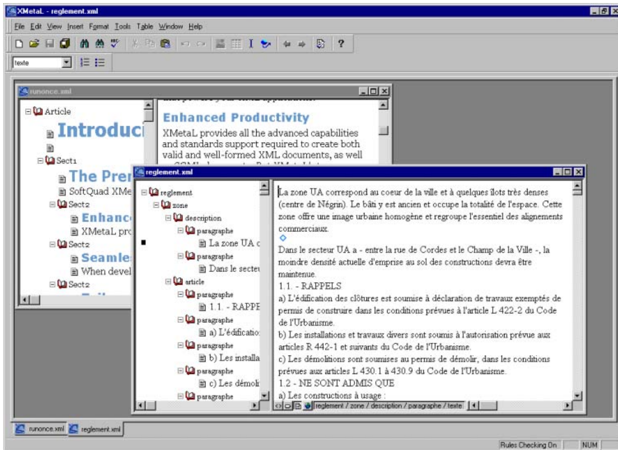
Figure 30 : XMetal
