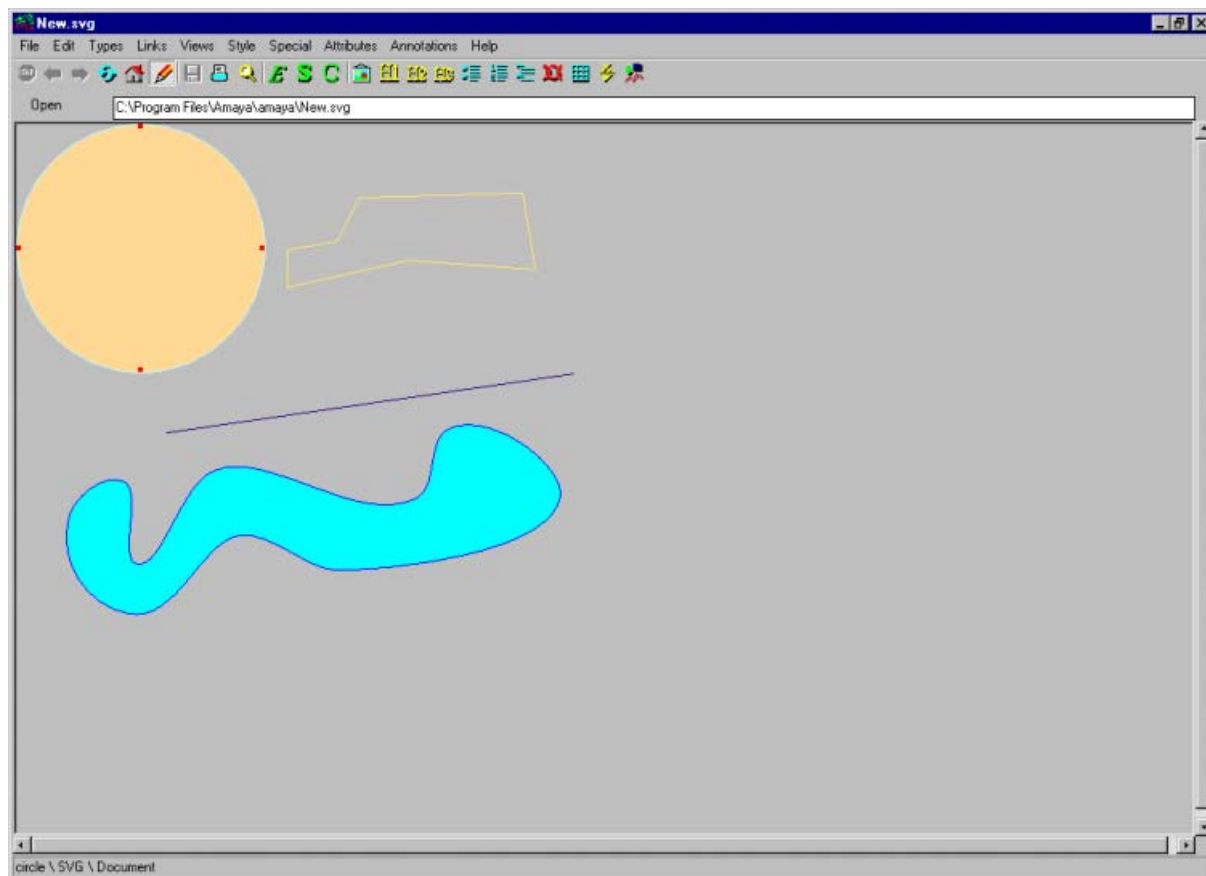
Figure 36 : W3C Amaya
