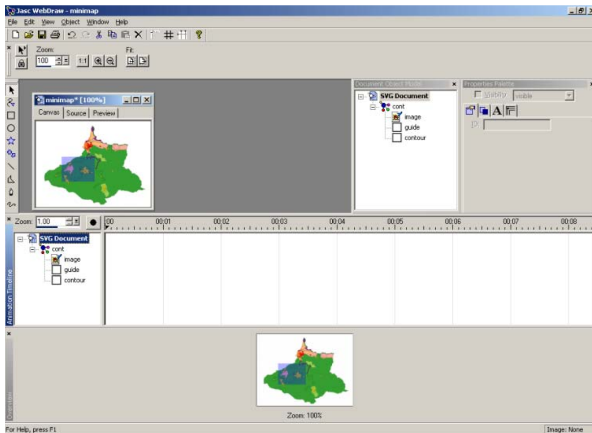
Figure 35 : Jasc WebDraw
