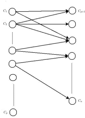
Figure 5: When the optimal plan is a bipartite graph.
