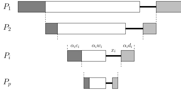
Figure 2: LIFO strategy. Dark grey rectangles (of length \alpha_i c_i ) represent the initial messages destined to the workers. White rectangles (of length \alpha_i w_i ) represent the computation on the workers. Light grey rectangles (of length \alpha_i d_i ) represent the return messages back to the master. Bold lines (of length x_i ) represent the idle time of the workers.
