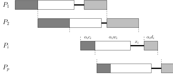
Figure 6: FIFO strategies.
