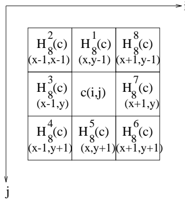
Figure 2.2: Moore's neighborhood.
