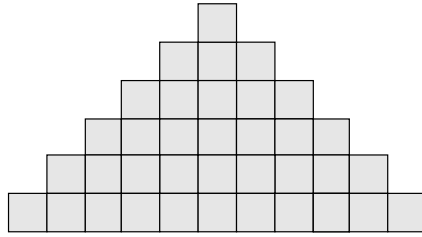
Figure 6.6: Isosceles triangle.
