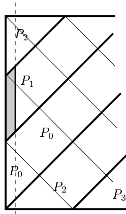
Figure 5: When the iteration-space is large, optimal tiling is made of diamond-shaped tiles. The presence of orthonormalization phase every 4n_{ortho} steps (represented by dash-line) explains the parallelogram shapes of tiles represented in Figure 6.
