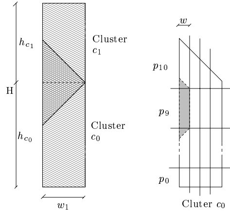
Figure 19: Hierarchical tiling for two clusters of processors. Here h_{c_1} = \frac{t_{seq}(c_0)}{t_{seq}(c_0)+t_{seq}(c_1)} and h_{c_0} = \frac{t_{seq}(c_1)}{t_{seq}(c_0)+t_{seq}(c_1)} .
