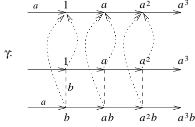
Figure 9: The homomorphism \gamma : \langle a, b \mid ab = ba, b^2 = 1 \rangle \rightarrow \langle a \mid \emptyset \rangle .
