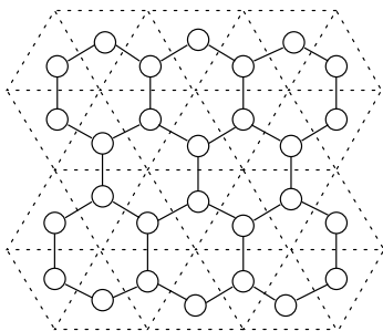
Figure 10: Triangular neighborhood.
