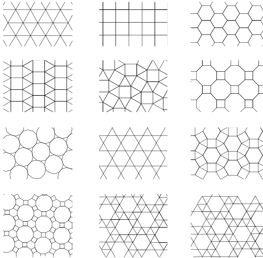
Figure 18: Archimedean tilings.
