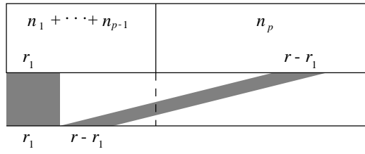
Figure 5: Generalized butterfly network case 1
