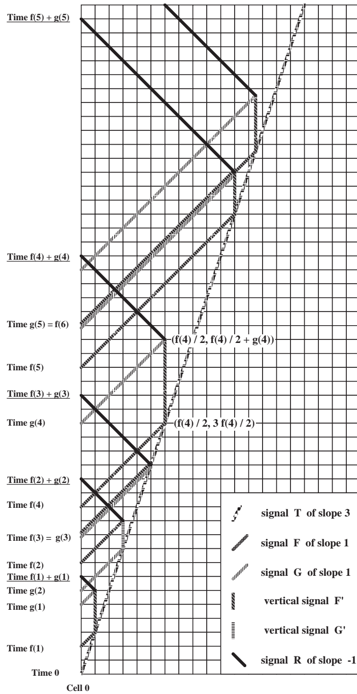
Figure 10: Fischer's construction of f + g .
