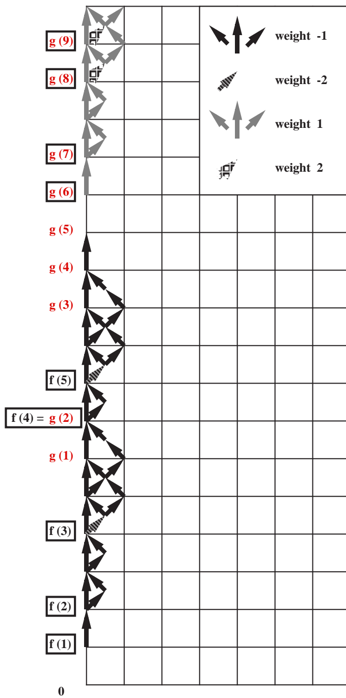
Figure 16: Fischer's construction of \min(f, g) .
