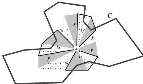
Figure 3: The intersection of the anti-yellow cycle C with S_x
