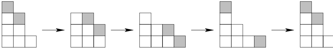
Figure 12: A circuit of (3, 2) -quasi-regular stairs on \mathcal{P}(8) .
