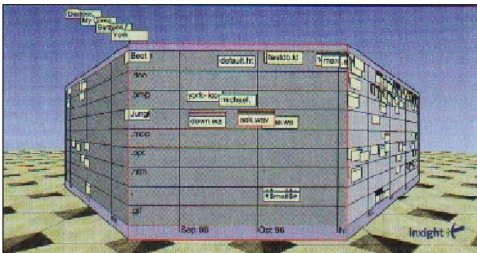
Perspective Wall
